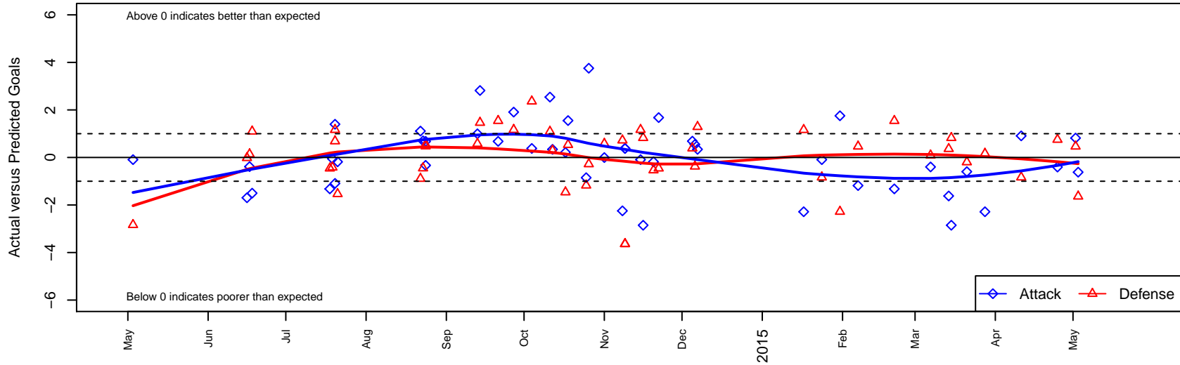
FC Alliance A B01 Dots are actual minus expected GF (blue circles) and GA (red triangles). Blue line is smoothed change in attack strength. Red is smoothed change in defense strength.
